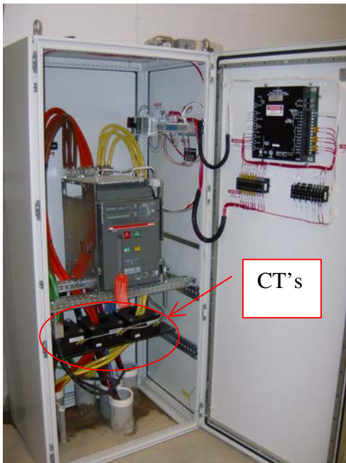
Electric Panel
