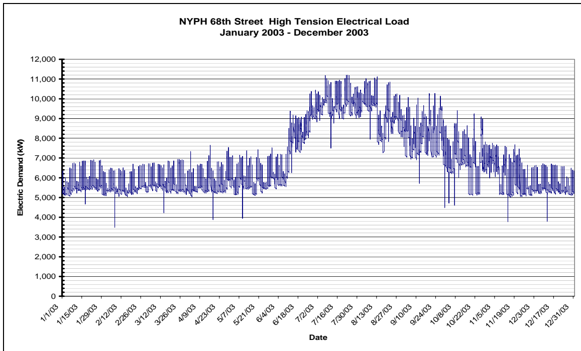
Figure 6 Annual Electricity Consumption of HT Service
