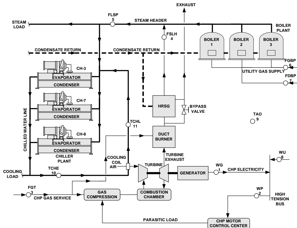
Figure 8 M&V Schematic
