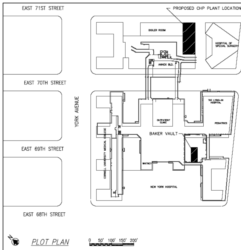
Figure 4 piping and raceways for Downtown Campus
