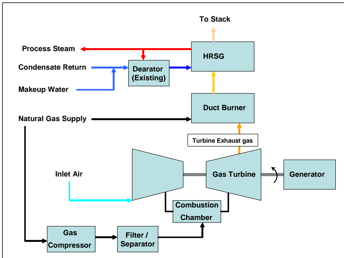
Figure 7 CHP System Schematic
