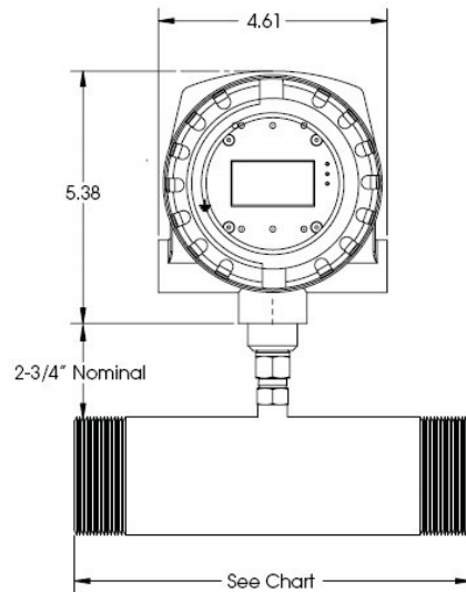
Sage SIP Flow Meter (FGE2) and (FGF2)
