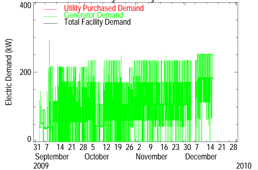
Facility Electricity Profile
