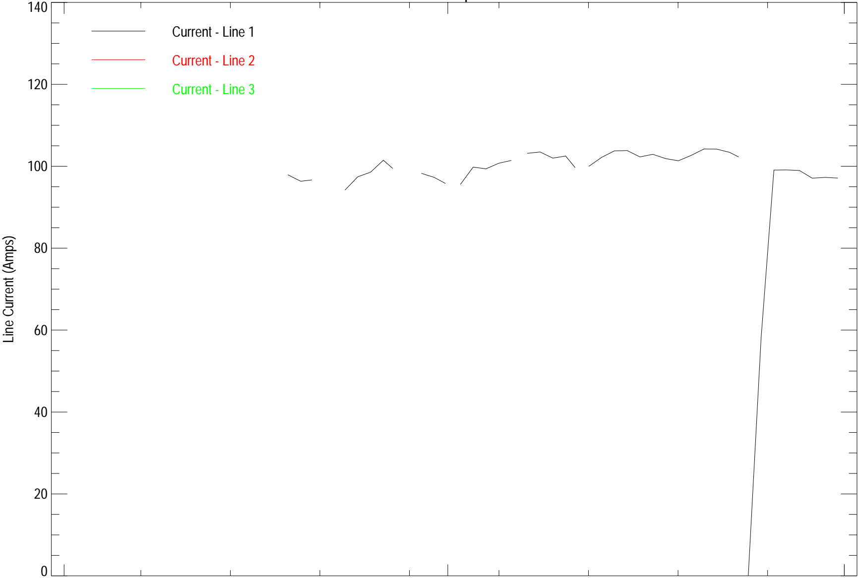
Generator Output Current
